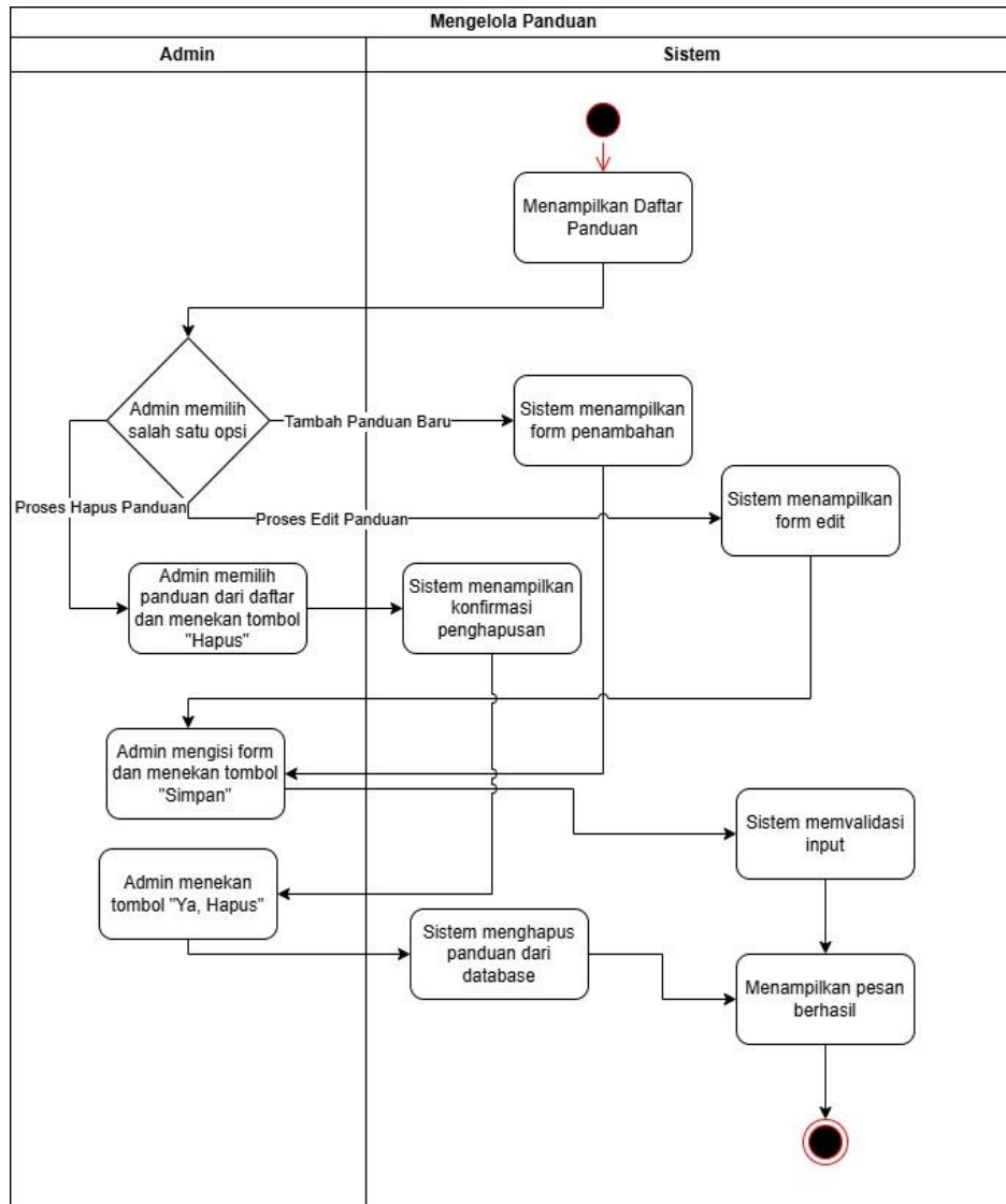
Gambar 1. 8 Activity Diagram Mengelola Panduan
