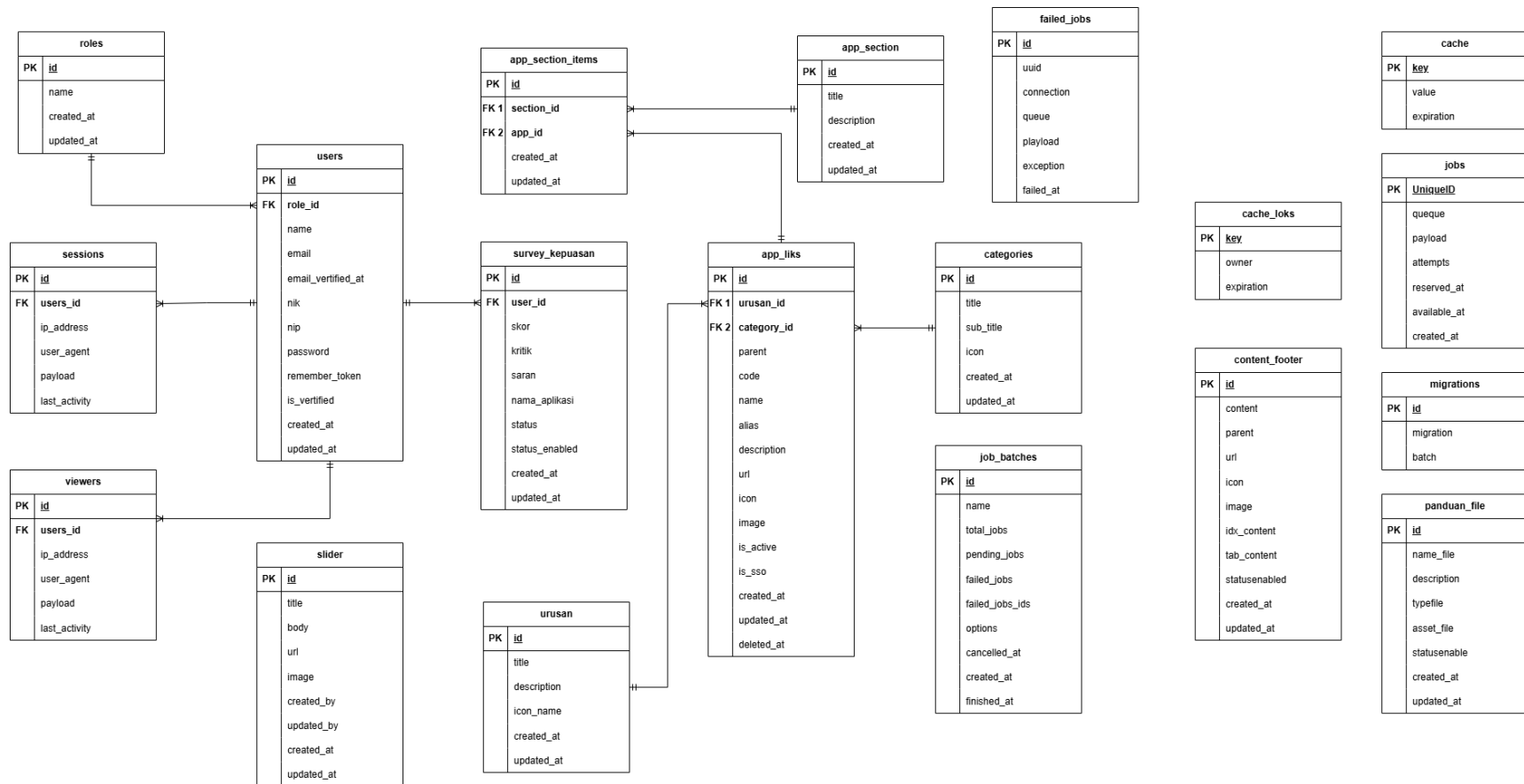
Gambar 1. 10 Entity Relationship Diagram
